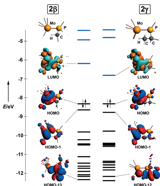
Figure 4. Energy level diagram for 2γ and 2β , with selected MOs depicted (isosurface value is 0.03). The double occupancies are only illustrated for the HOMOs. Only the atoms of the agostic Mo–P–C(C)–H moieties are drawn as balls.
